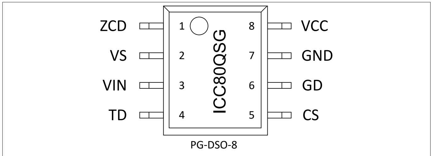
Figure 2 Pin configuration
