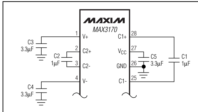
Figure 6. Charge-Pump Connections
