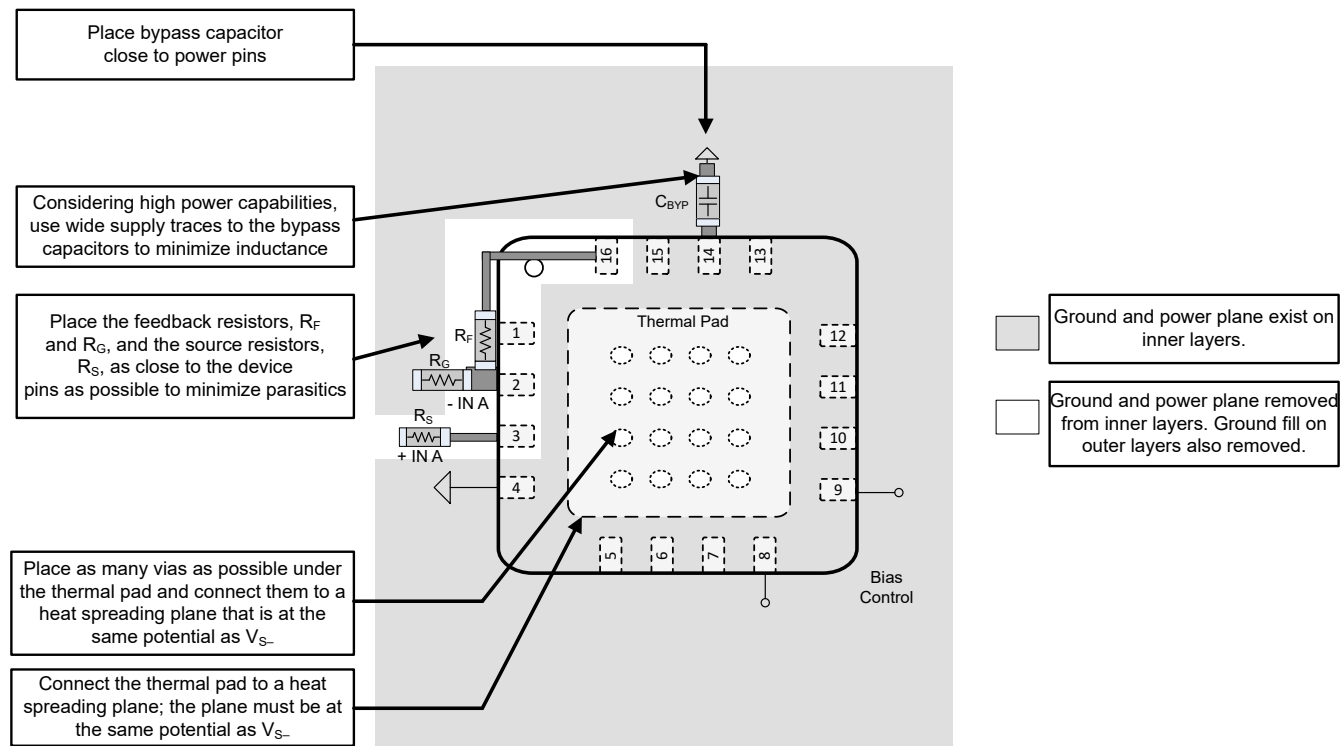
Figure 9-4. Layout Recommendations
