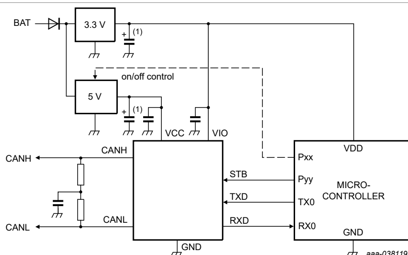
Figure 10. Typical TJR1442A application with a 3.3 V microcontroller
