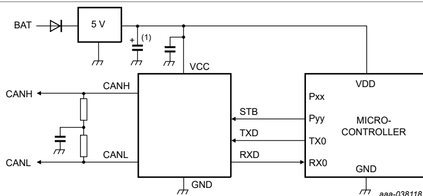
Figure 11. Typical TJR1442B application with a 5 V microcontroller
