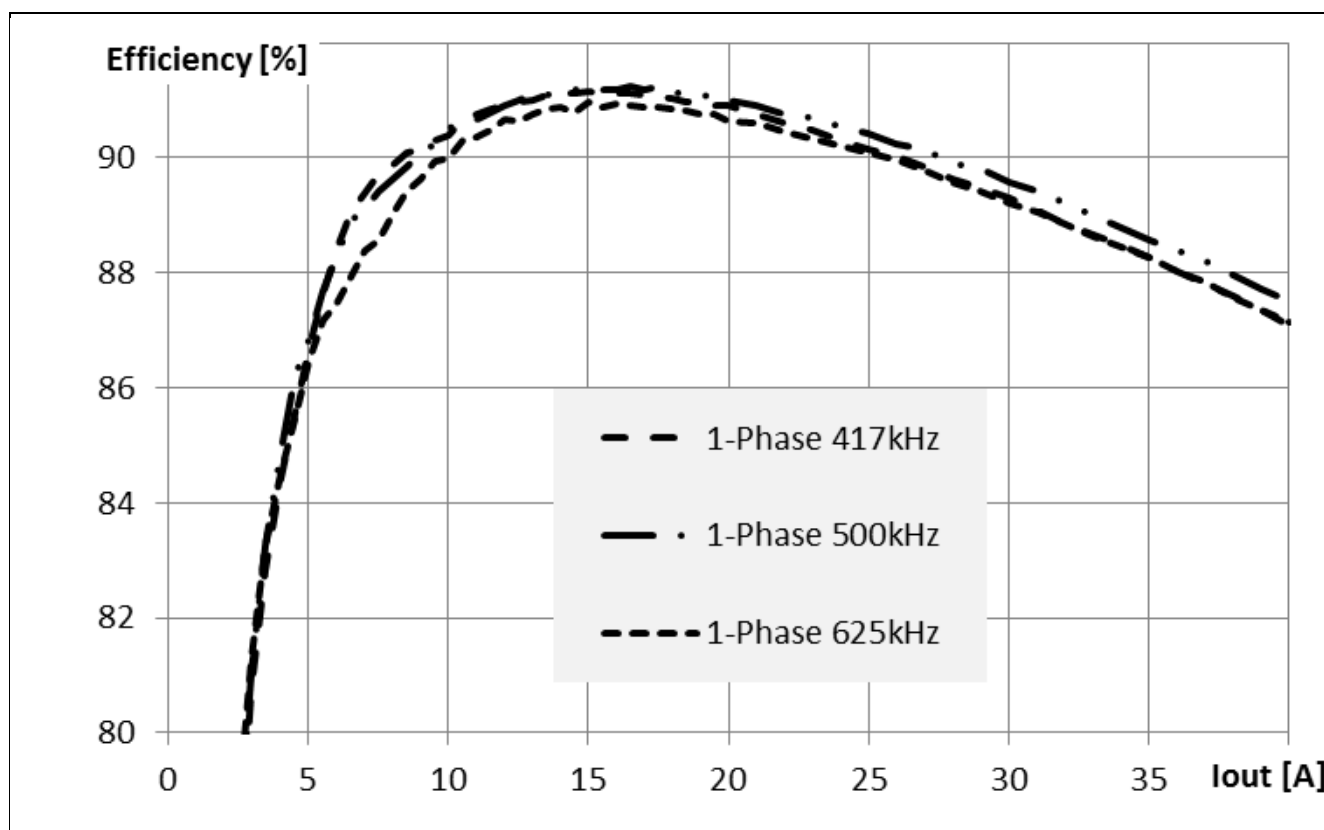
Figure 15 Efficiency at VIN = 12 V, VCC = PVCC = 5 V, Single Phase, VOUT = 1.2 V
