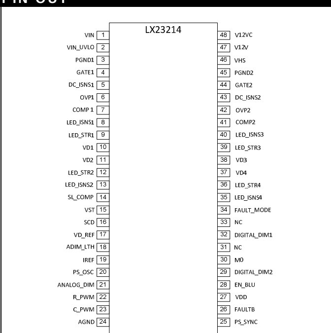
Figure 2: LX23214IDB SSOP Package Pin Out
