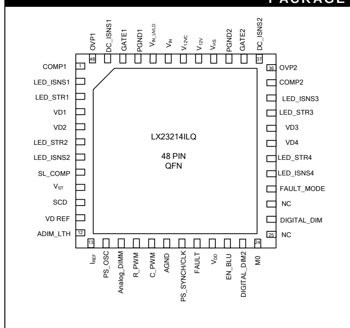
Figure 1: LX23214ILQ QFN Package Pin Out
