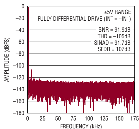
Figure 7c. IN^+/IN^- = 450\text{mV} 200Hz Fully Differential Sine, 0\text{V} \leq V_{CM} \leq 24\text{V} , 32k Point FFT, f_{SAMPL} = 350\text{ksps} . Circuit Shown in Figure 7a
