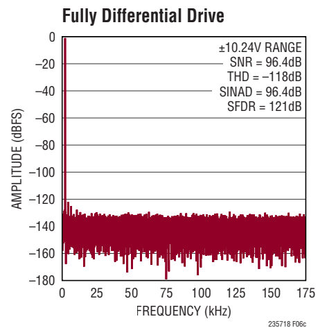
Figure 6c. IN^+/IN^- = -1\text{dBFS} 2kHz Fully Differential Sine, V_{\text{CM}} = 0\text{V} , 32k Point FFT, f_{\text{SAMPL}} = 350\text{ksps} . Circuit Shown in Figure 6a
