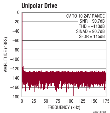
Figure 6e. IN^+ = -1\text{dBFS} 2kHz Unipolar Sine, IN^- = 0\text{V} , 32k Point FFT, f_{\text{SAMPL}} = 350\text{ksps} . Circuit Shown in Figure 6a
