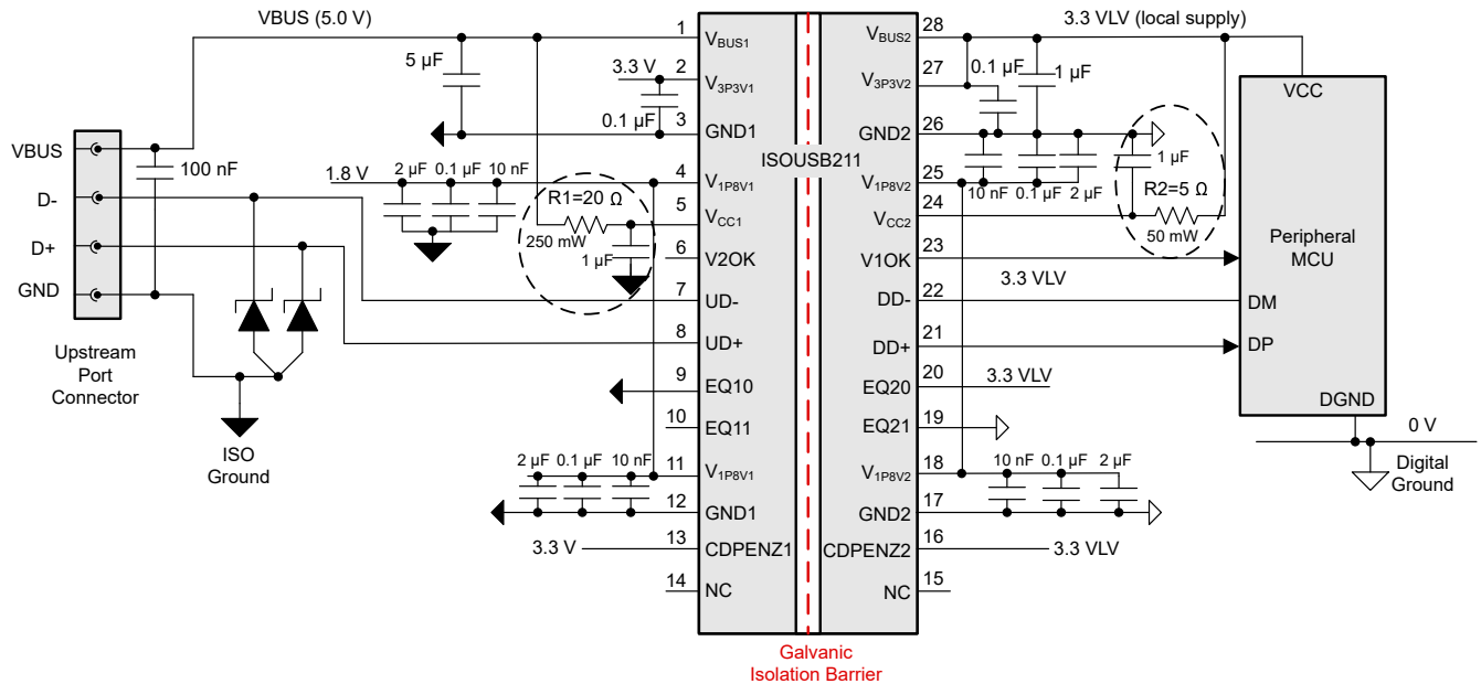
Figure 10-8. Using ISOUUSB211 with Resistors in series with V CCx pins
