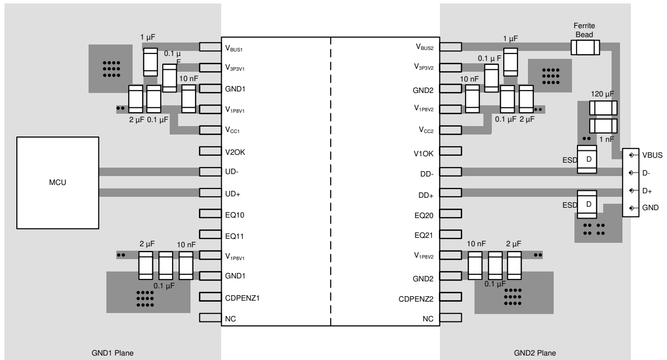
Figure 11-1. Layout Example for ISOUUSB211
