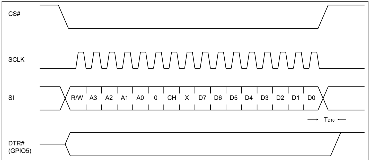
Figure 11. SPI Write MCR To DTR Output Switch
