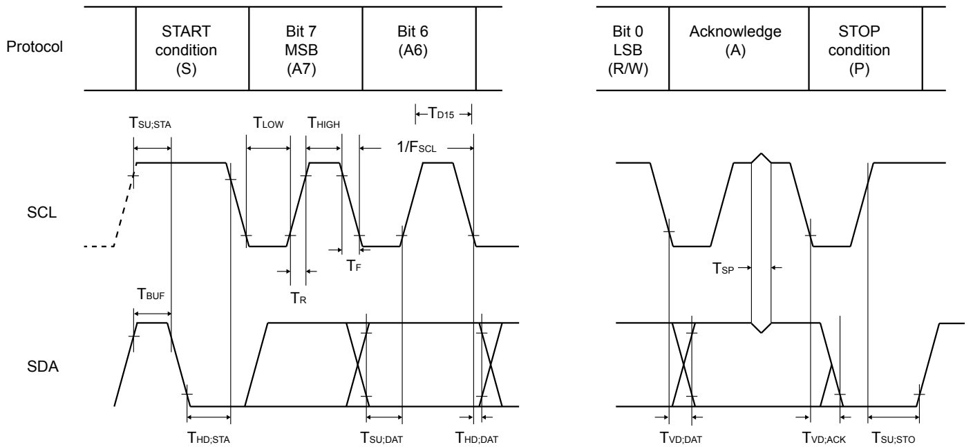
Figure 2. I²C-Bus Timing Diagram
