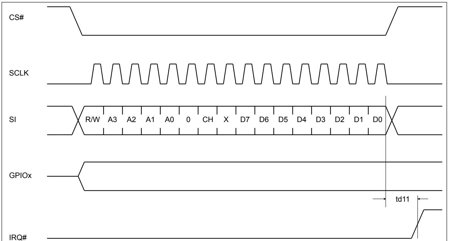
Figure 12. SPI Write THR To Clear TX INT
