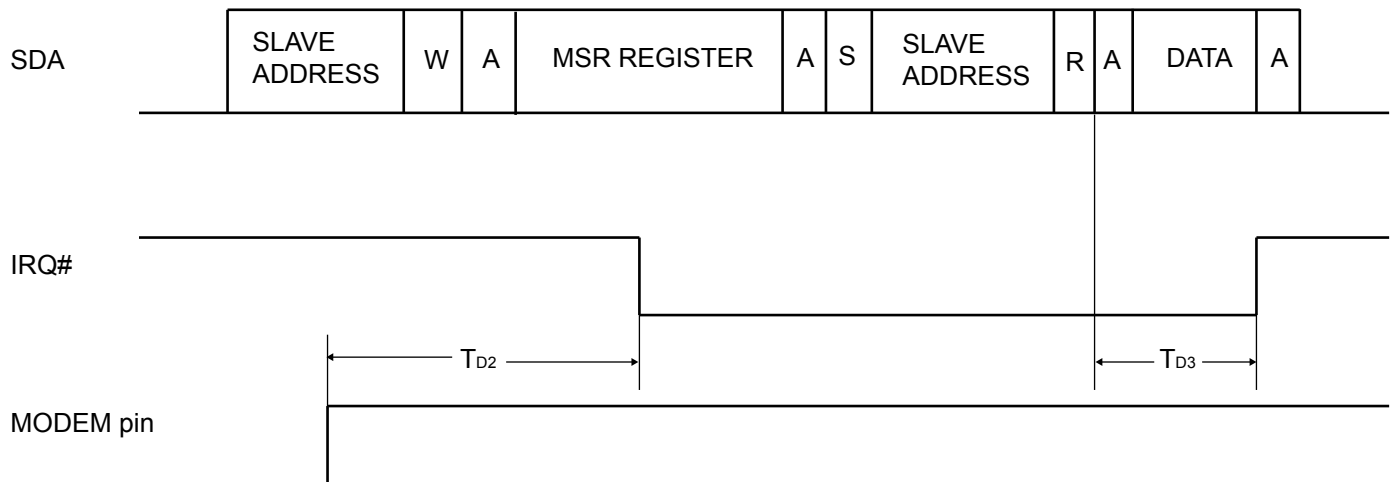
Figure 4. Modem Input Pin Interrupt
