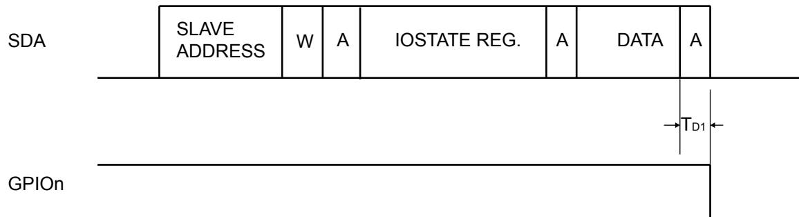
Figure 3. Write To Output
