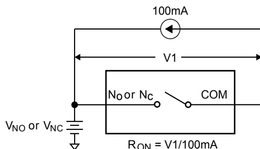
Figure 1. On Resistance
