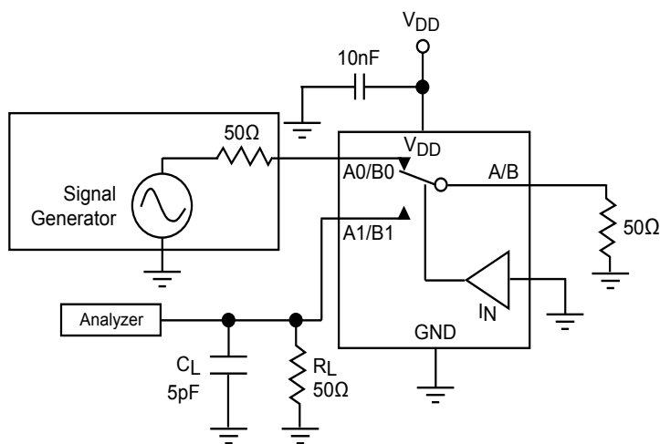
Figure 5. Input Isolation
