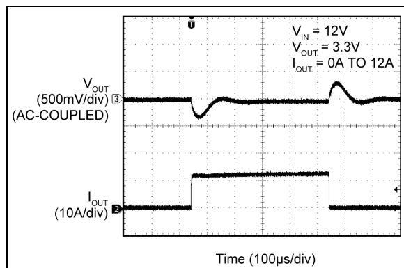
FIGURE 2-79: MIC2102 Transient Response.
