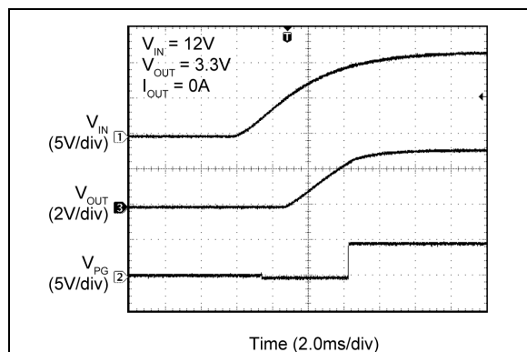
FIGURE 2-81: Power Good at V_{IN} Soft Turn-On.
