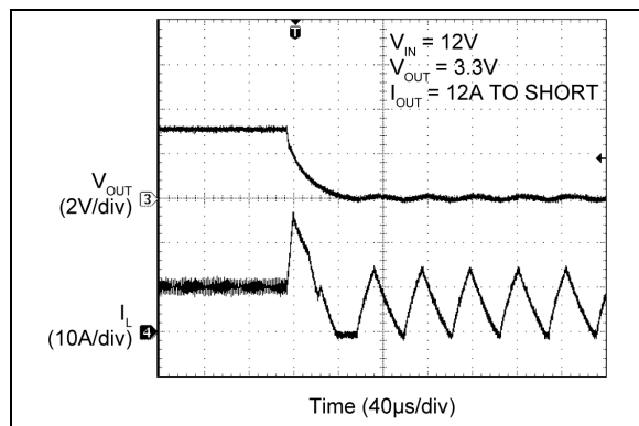
FIGURE 2-67: Short-Circuit.
