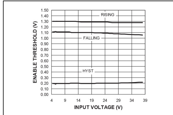
FIGURE 2-46: Enable Threshold vs. Input Voltage.
