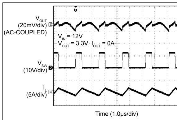
FIGURE 2-72: MIC2102 Switching Waveforms ( I_{OUT} = 0A ).
