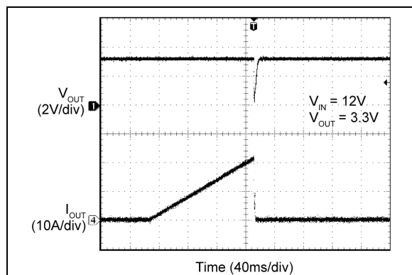
FIGURE 2-69: Output Peak Current-Limit Threshold.
