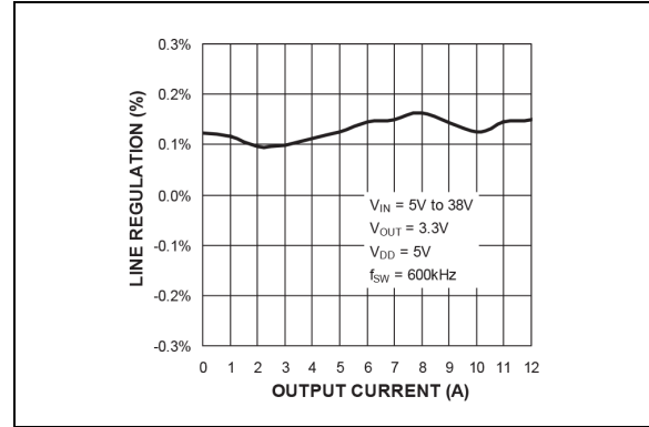
FIGURE 2-30: Line Regulation vs. Output Current (MIC2102).
