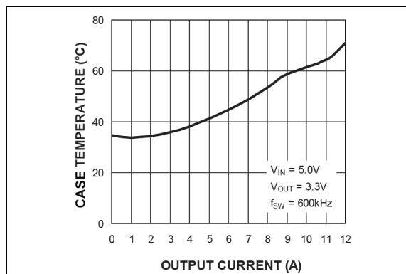
FIGURE 2-36: Case Temperature* ( V_{IN} = 5.0V ) vs. Output Current.
