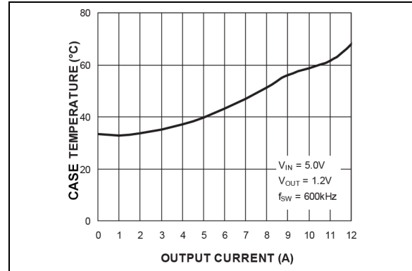
FIGURE 2-40: Case Temperature* ( V_{IN} = 5.0V ) vs. Output Current.
