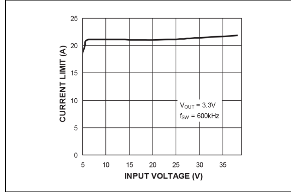
FIGURE 2-48: Output peak Current Limit vs. Input Voltage.
