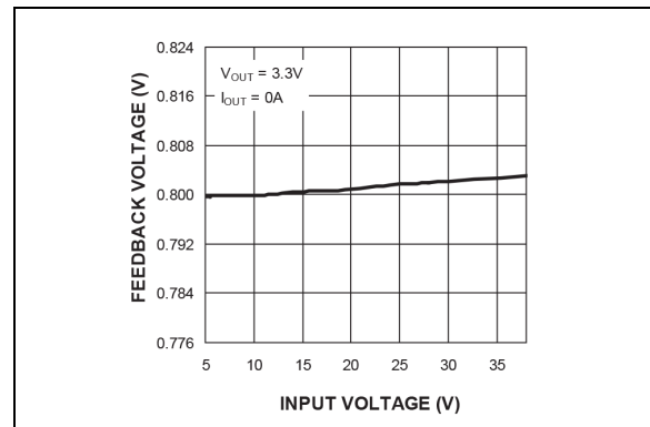
FIGURE 2-5: Feedback Voltage vs. Input Voltage (MIC2101).
