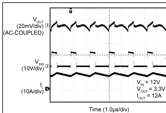
FIGURE 2-71: MIC2102 Switching Waveforms ( I_{OUT} = 12A ).
