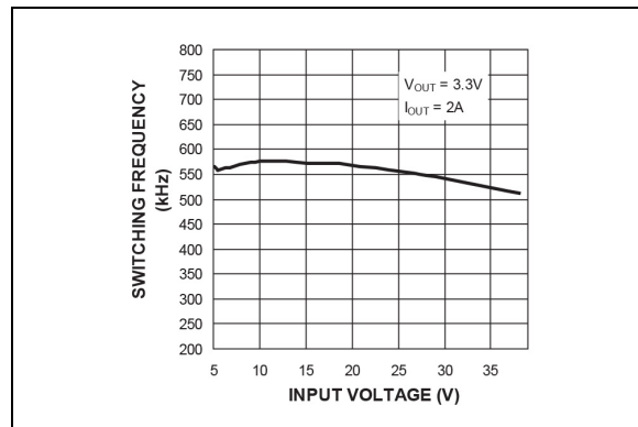
FIGURE 2-47: Switching Frequency vs. Input Voltage.
