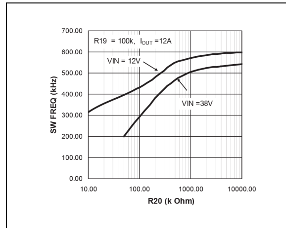
FIGURE 5-2: Switching Frequency vs. R20.
