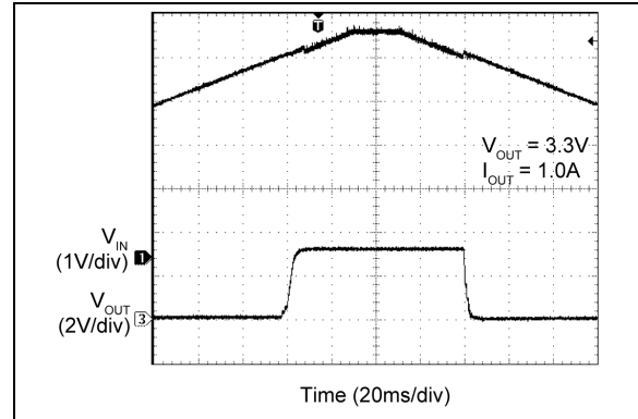
FIGURE 2-64: V_{IN} UVLO Thresholds.
