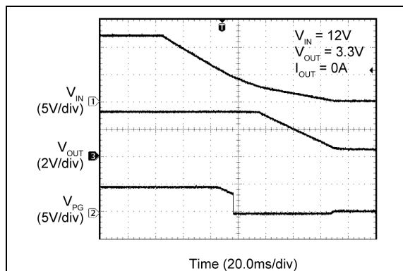
FIGURE 2-82: Power Good at V_{IN} Soft Turn-Off.
