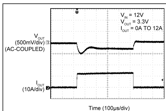
FIGURE 2-80: MIC2101 Transient Response.
