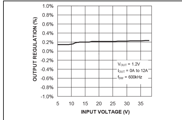
FIGURE 2-22: Output Regulation vs. Input Voltage (MIC2102).
