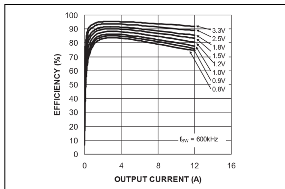
FIGURE 2-31: Efficiency ( V_{IN} = 5V ) vs. Output Current (MIC2102).
