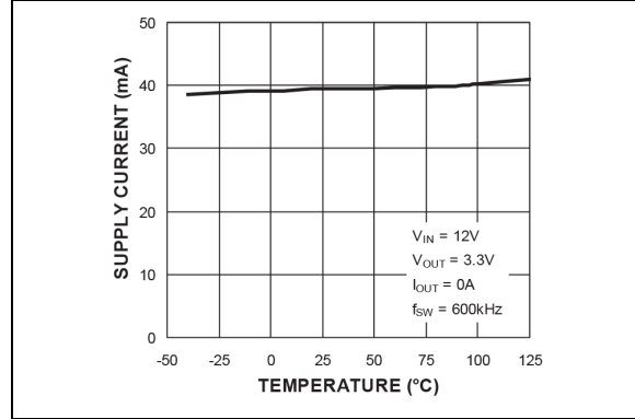
FIGURE 2-24: V_{IN} Operating Supply Current vs. Temperature (MIC2102).
