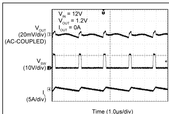
FIGURE 2-84: MIC2102 Switching Waveforms ( I_{OUT} = 0A ).
