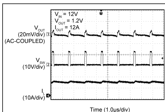
FIGURE 2-83: MIC2102 Switching Waveforms ( I_{OUT} = 12A ).
