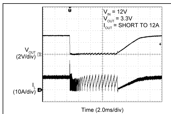
FIGURE 2-68: Output Recovery from Short Circuit.
