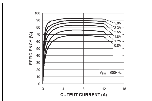
FIGURE 2-33: Efficiency ( V_{IN} = 18V ) vs. Output Current (MIC2102).
