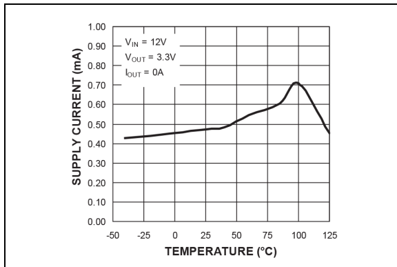
FIGURE 2-8: V IN Operating Supply Current vs. Temperature (MIC2101).
