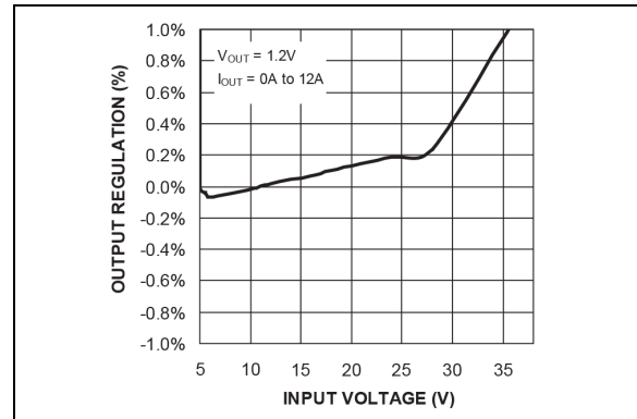
FIGURE 2-4: Output Regulation vs. Input Voltage (MIC2101).
