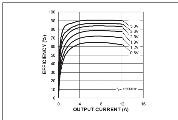
FIGURE 2-34: Efficiency ( V_{IN} = 24V ) vs. Output Current (MIC2102).
