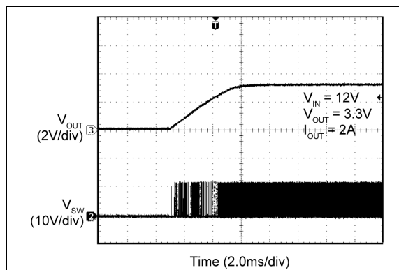
FIGURE 2-70: Output Recovery from Thermal Shutdown.
