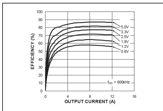
FIGURE 2-35: Efficiency ( V_{IN} = 38V ) vs. Output Current (MIC2102).
