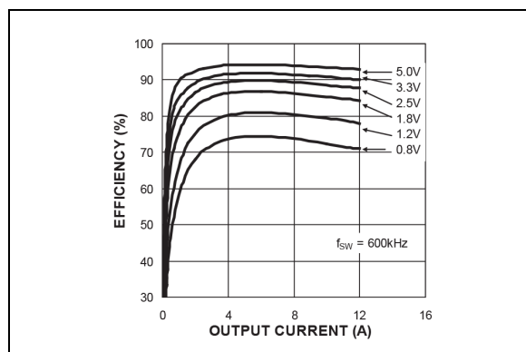
FIGURE 2-32: Efficiency ( V_{IN} = 12V ) vs. Output Current (MIC2102).
