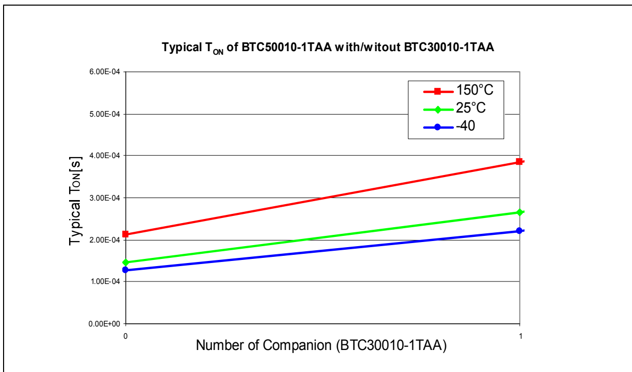
Figure 21 T_{ON} of BTC50010-1TAA with/without BTC30010-1TAA
