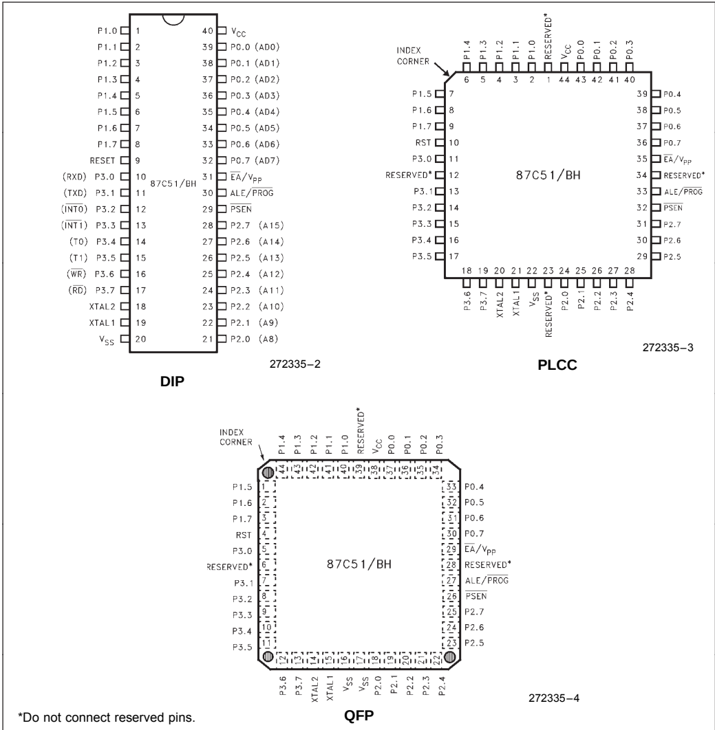
Figure 2. Pin Connections
