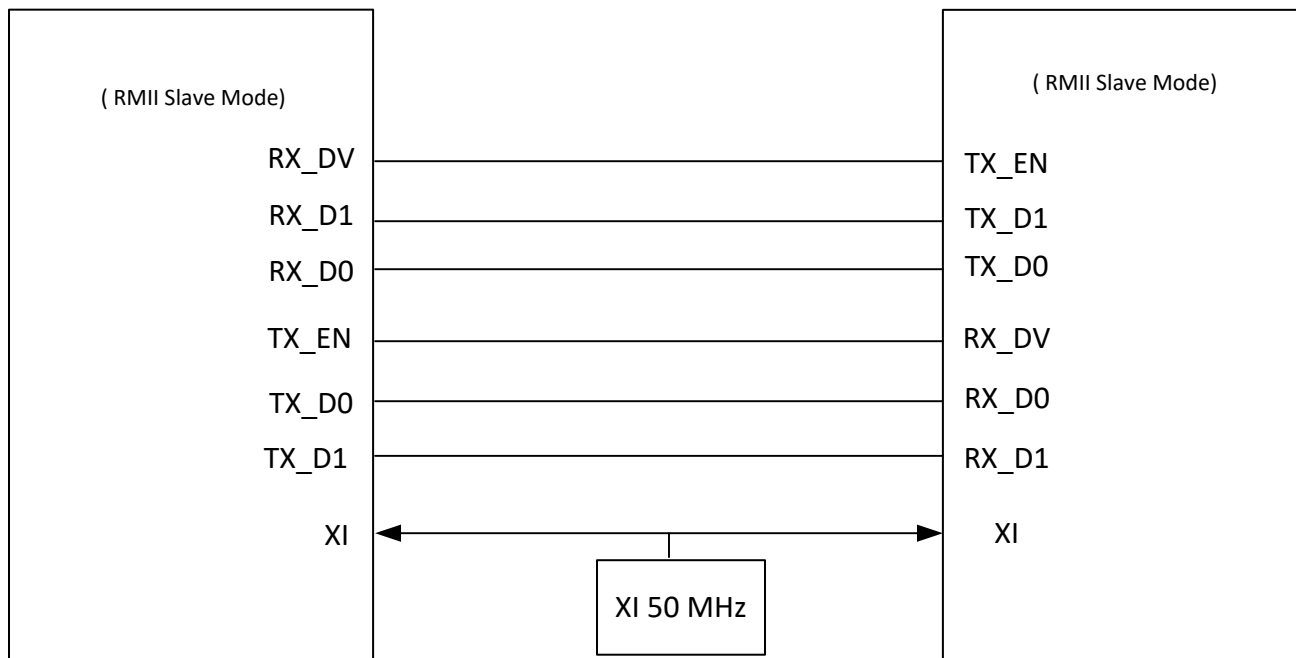
Figure 7-1. RMII Repeater Mode
