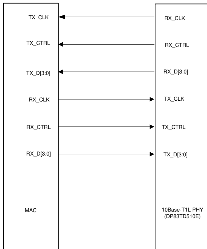
Figure 7-7. RGMII Signalling
