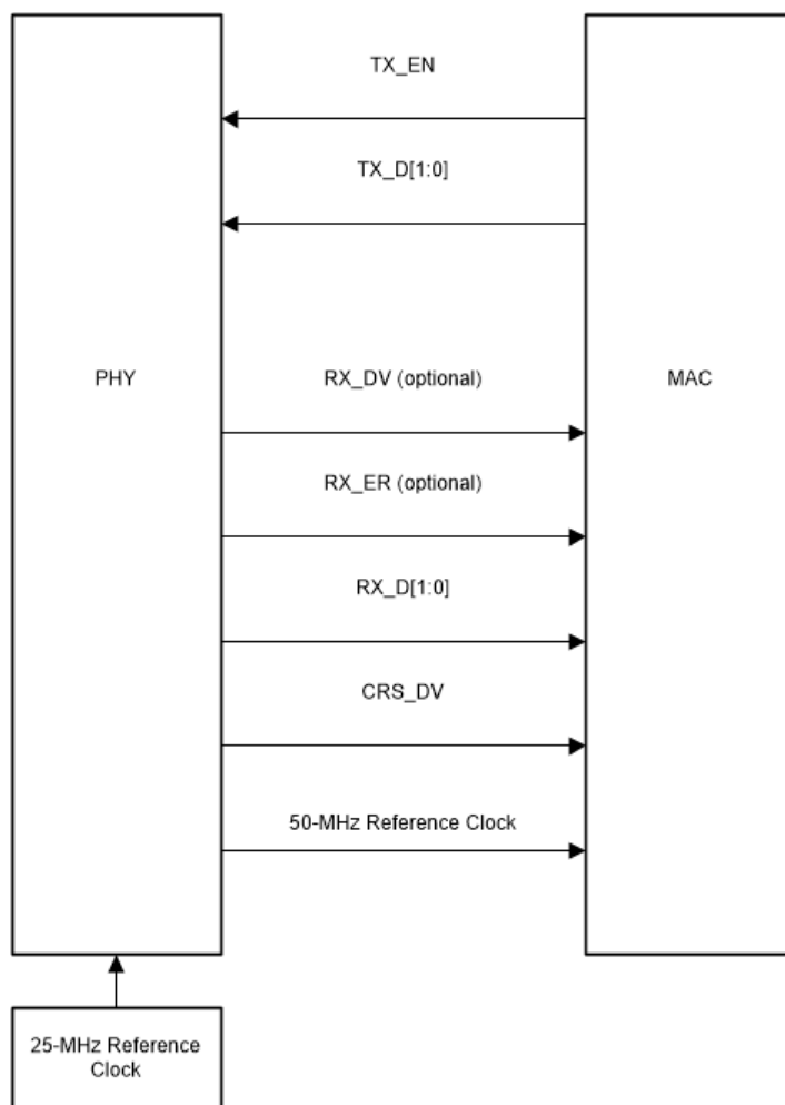
Figure 7-6. RMII Master Signaling
