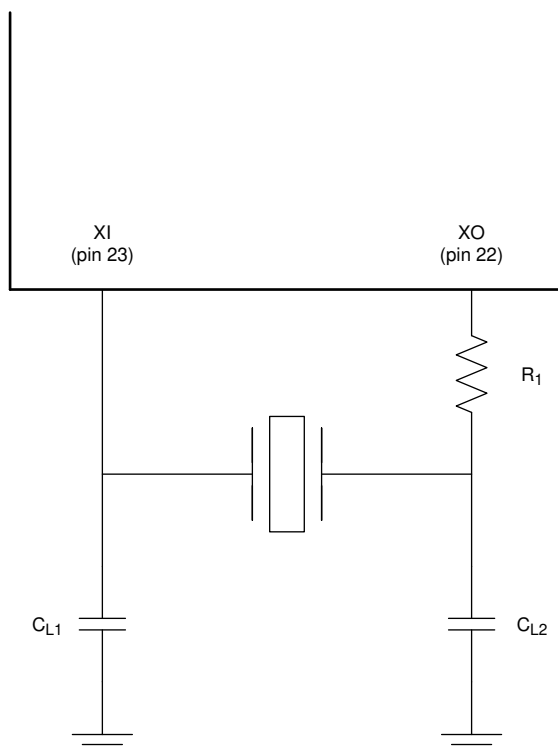
Figure 8-4. Crystal Oscillator Circuit
