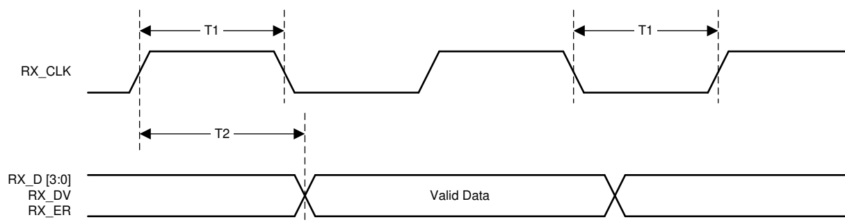
Figure 6-5. 10-Mbps MII Receive Timing
