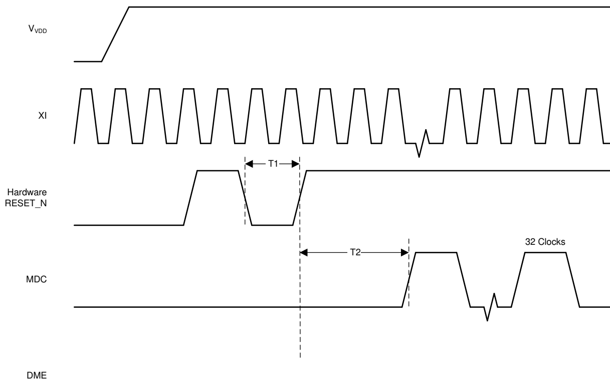
Figure 6-2. Reset Timing
