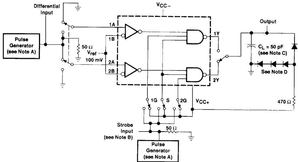
TEST CIRCUIT
