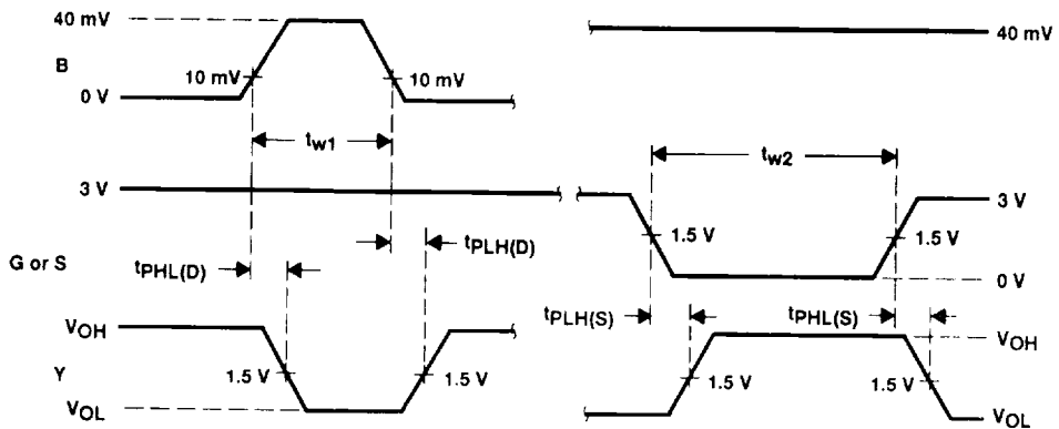
VOLTAGE WAVEFORMS
