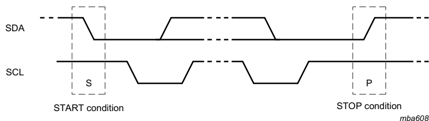
Fig 8. Definition of START and STOP conditions
