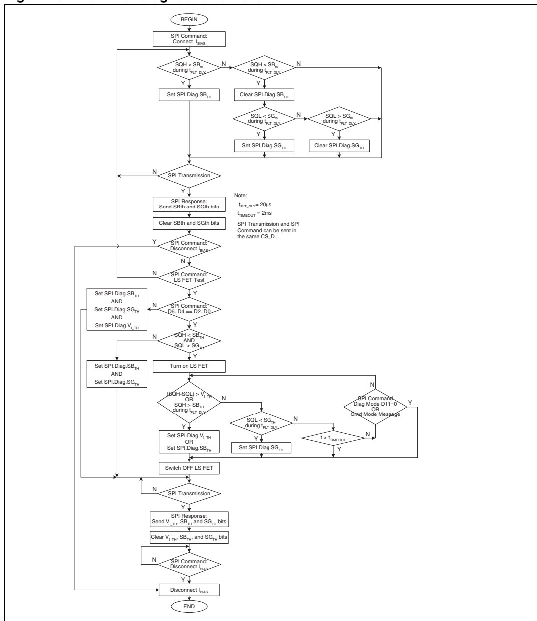
Figure 16. Low side diagnostic flow chart
