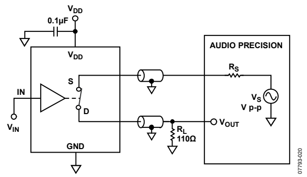
Figure 18. THD + Noise
