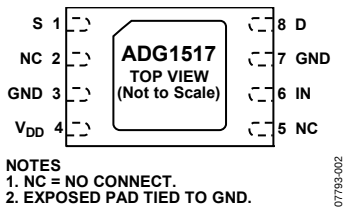
Figure 2. Pin Configuration
