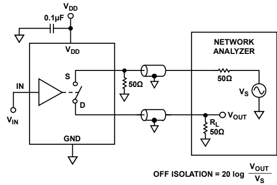
Figure 16. Off Isolation
