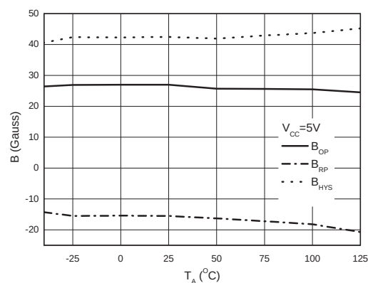
Figure 10. B_{OP}/B_{RP}/B_{HYS} vs. T_A ( V_{CC}=5V )
