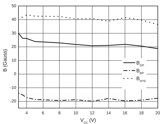
Figure 9. B_{OP}/B_{RP}/B_{HYS} vs. V_{CC}
