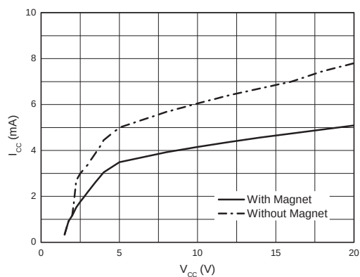
Figure 7. I_{CC} vs. V_{CC}
