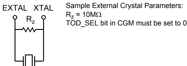
Figure 4-6 Crystal Oscillator
