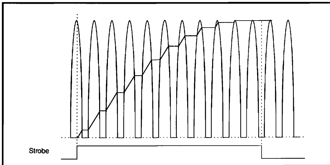
FIGURE 8: Servo Burst Acquisition (SG = RESET = 1)
