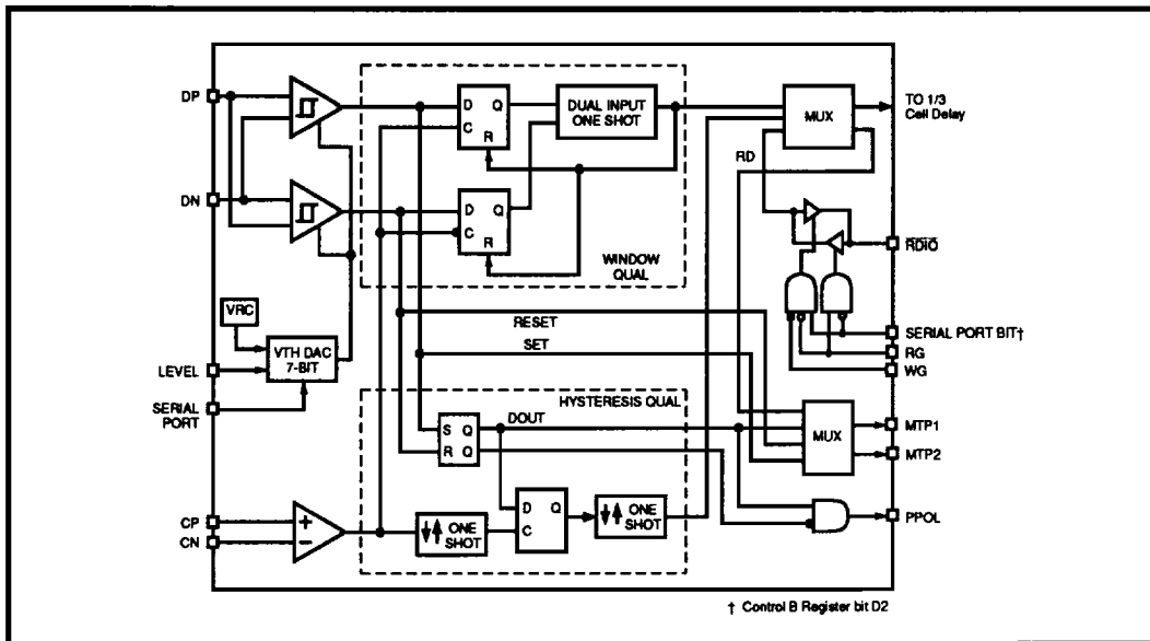
FIGURE 3: Pulse Qualification
