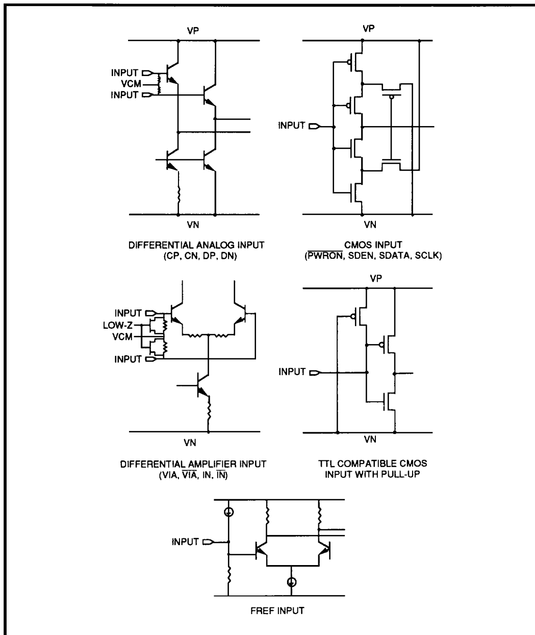
FIGURE 17: Input Structures
