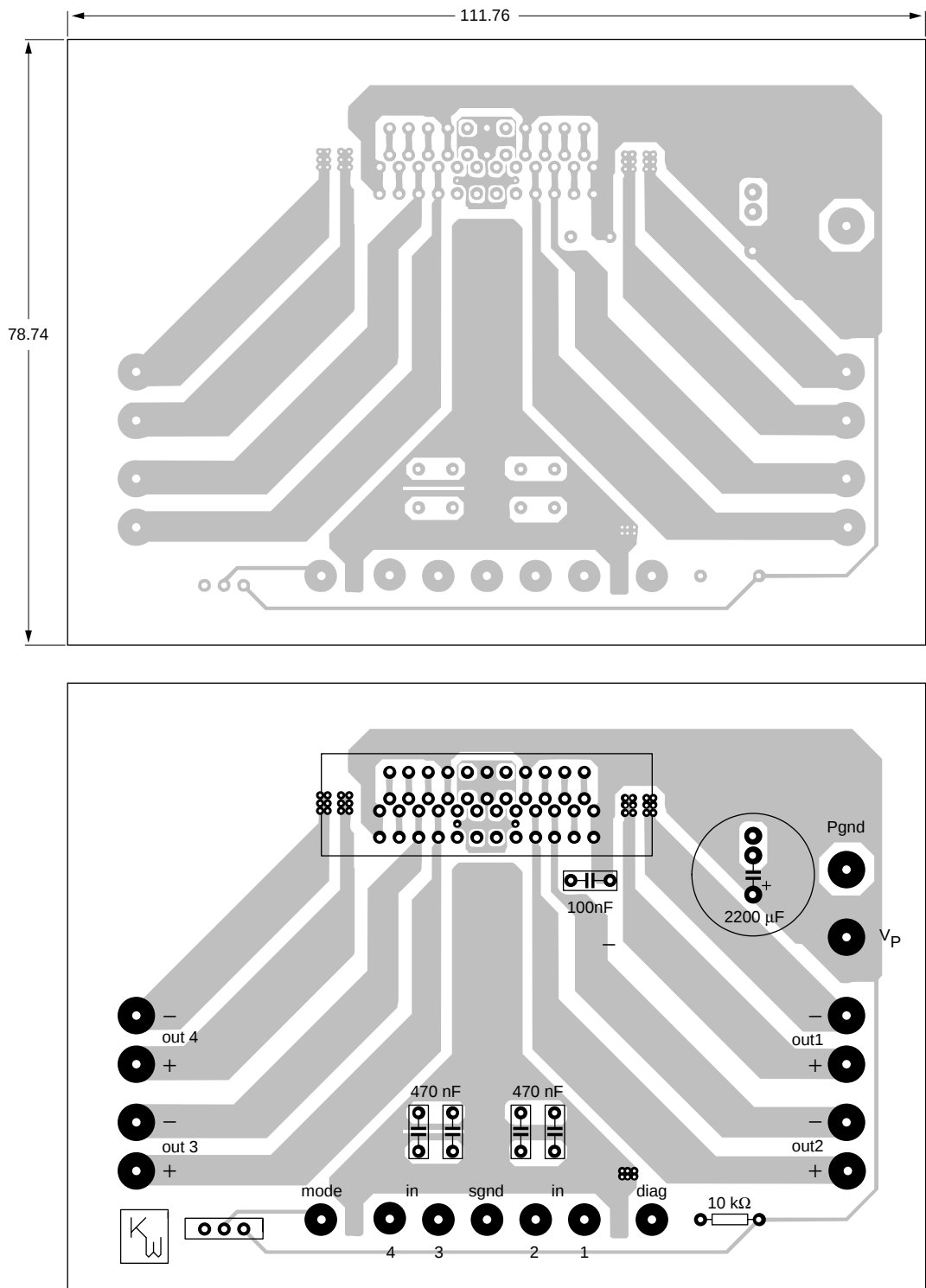
Fig.15 PCB layout (soldering side).
