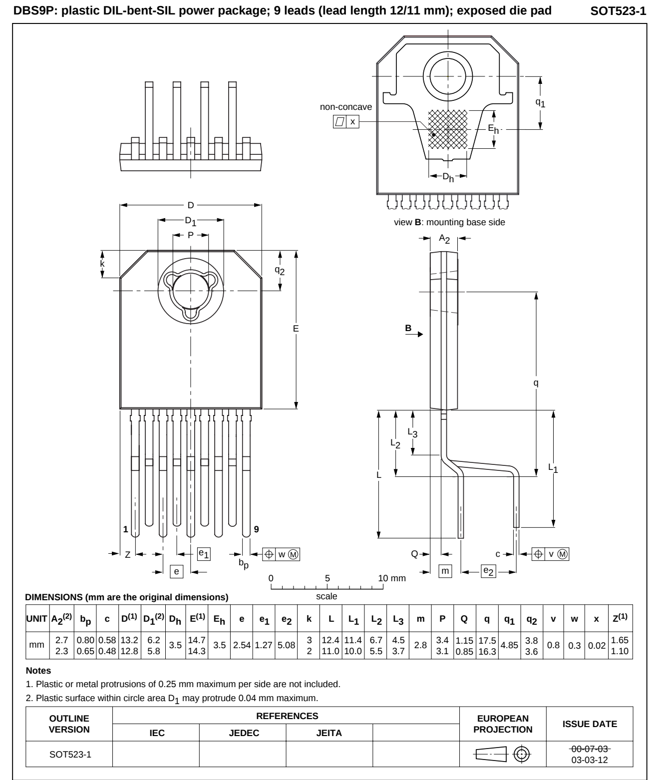
Fig 15. Package outline.
