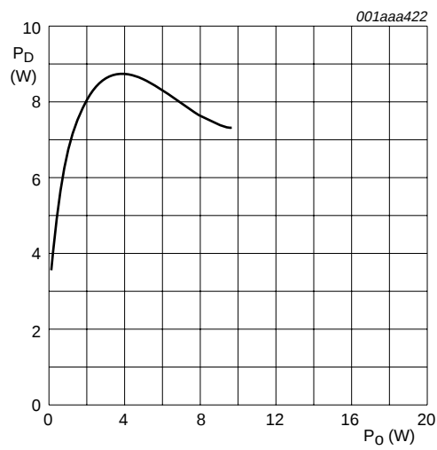
Fig 9. Total (worst-case, both channels driven) power dissipation as function of channel output power per channel.
