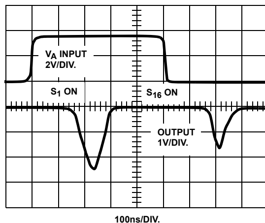
FIGURE 6C. WAVEFORMS
