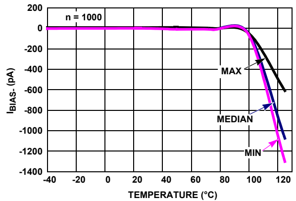
FIGURE 23. I_{BIAS-} vs TEMPERATURE V_+ = 5V , V_- = 0V
