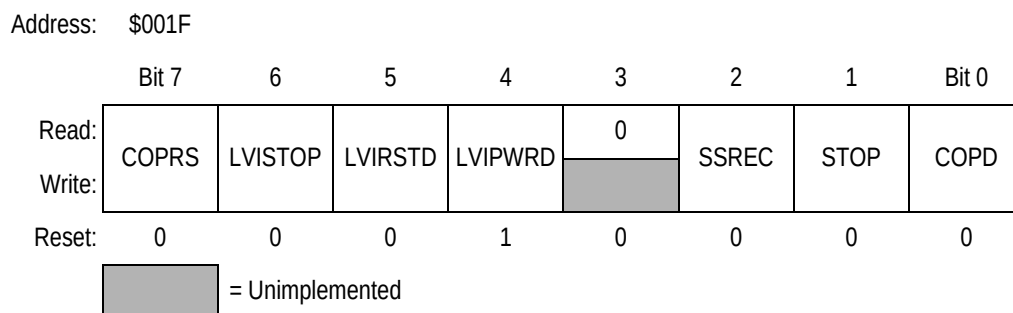
Figure 20-2. Configuration Register 1 (CONFIG1)
