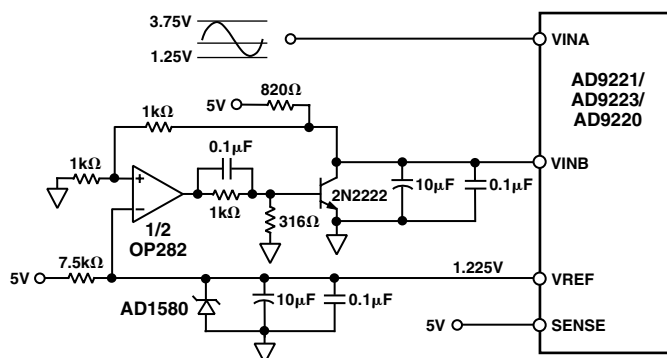
Figure 26. External Reference Using the AD1580 and Low Impedance Buffer
