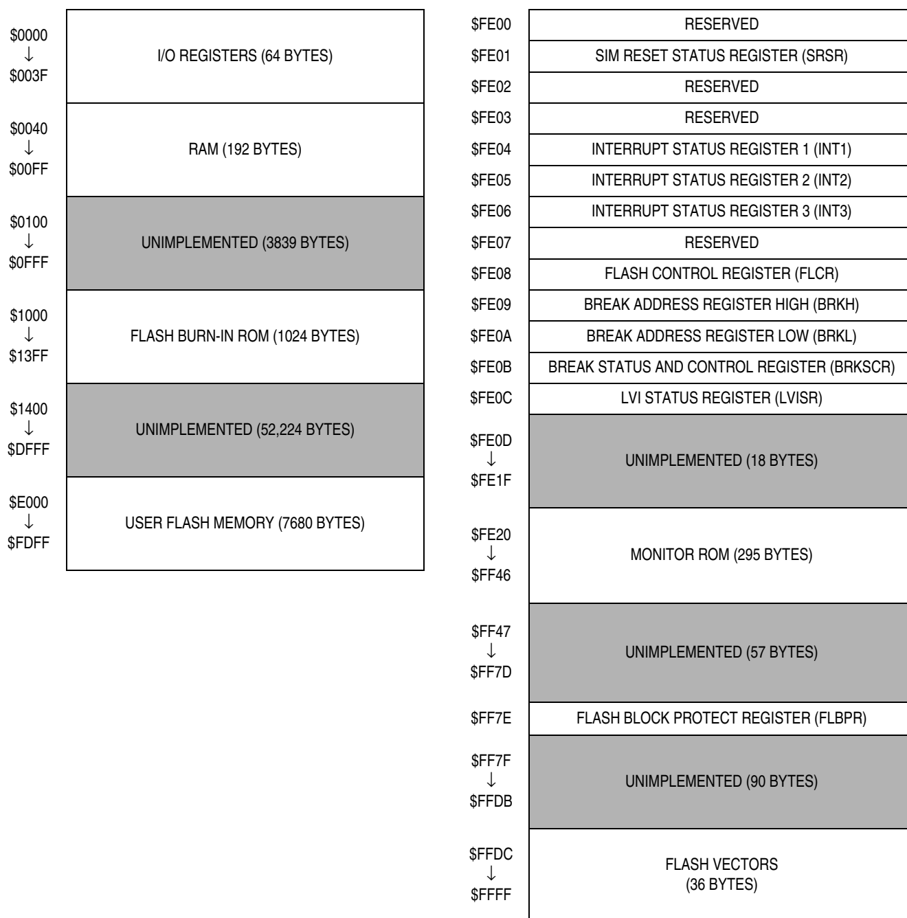
Figure 2-1. Memory Map
