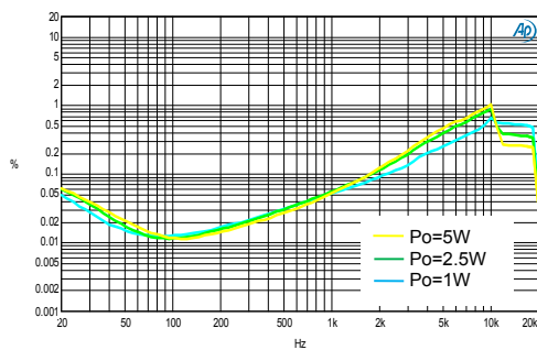
THD + N vs. Frequency 18V, 8\Omega + 66\mu\text{H}
