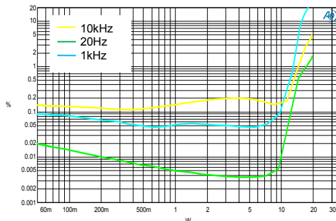
THD + N vs. P OUT 16V, 8\Omega + 66\mu\text{H}
