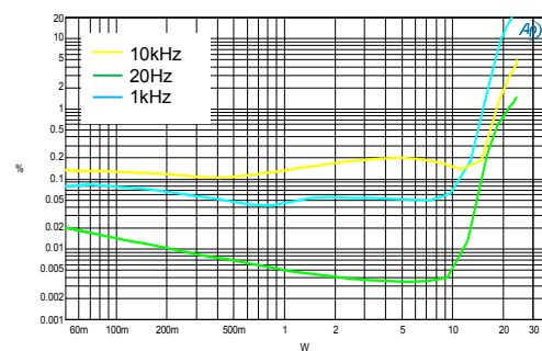
THD + N vs. P OUT 18V, 8\Omega + 66\mu\text{H}
