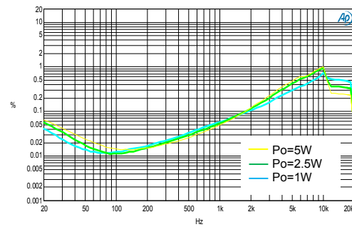
THD + N vs. Frequency 16V, 8\Omega + 66\mu\text{H}
