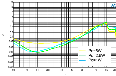
THD + N vs. Frequency 12V, 8\Omega + 66\mu\text{H}
