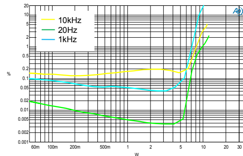
THD + N vs. P OUT 12V, 8\Omega + 66\mu\text{H}
