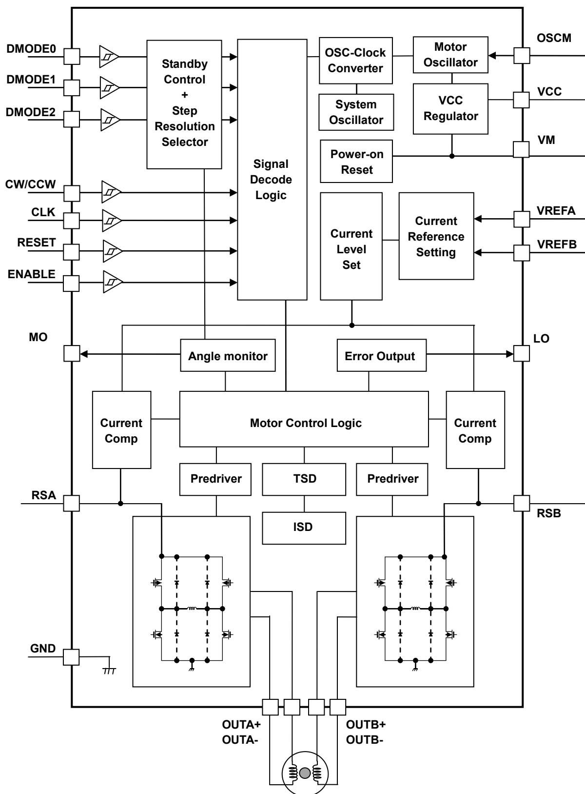
TB67S269 Block diagram
