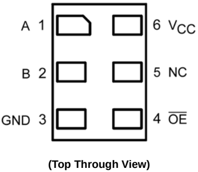
Pad Assignments for MicroPak
