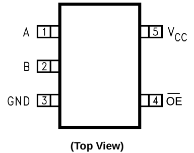
Pad Assignments for MicroPak
