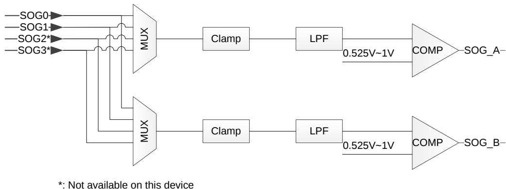
Figure 3.3. Sync Slicers
