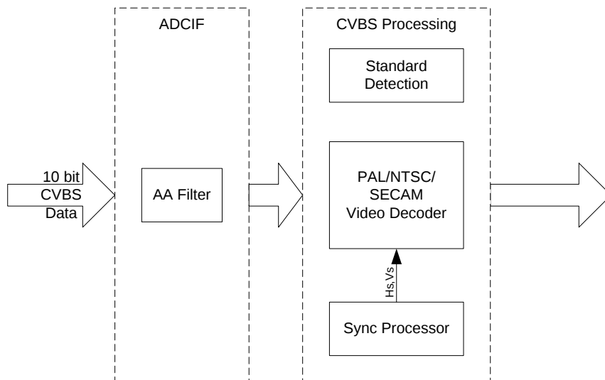
Figure 3.4. CVBS Processing Diagram
