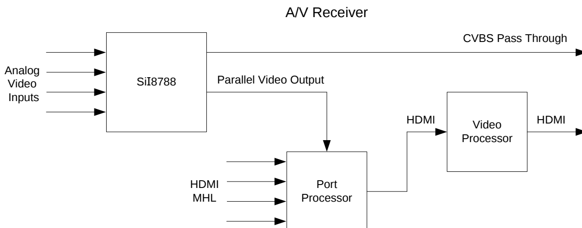
Figure 1.1. Typical Application of the SiI8788 Device
