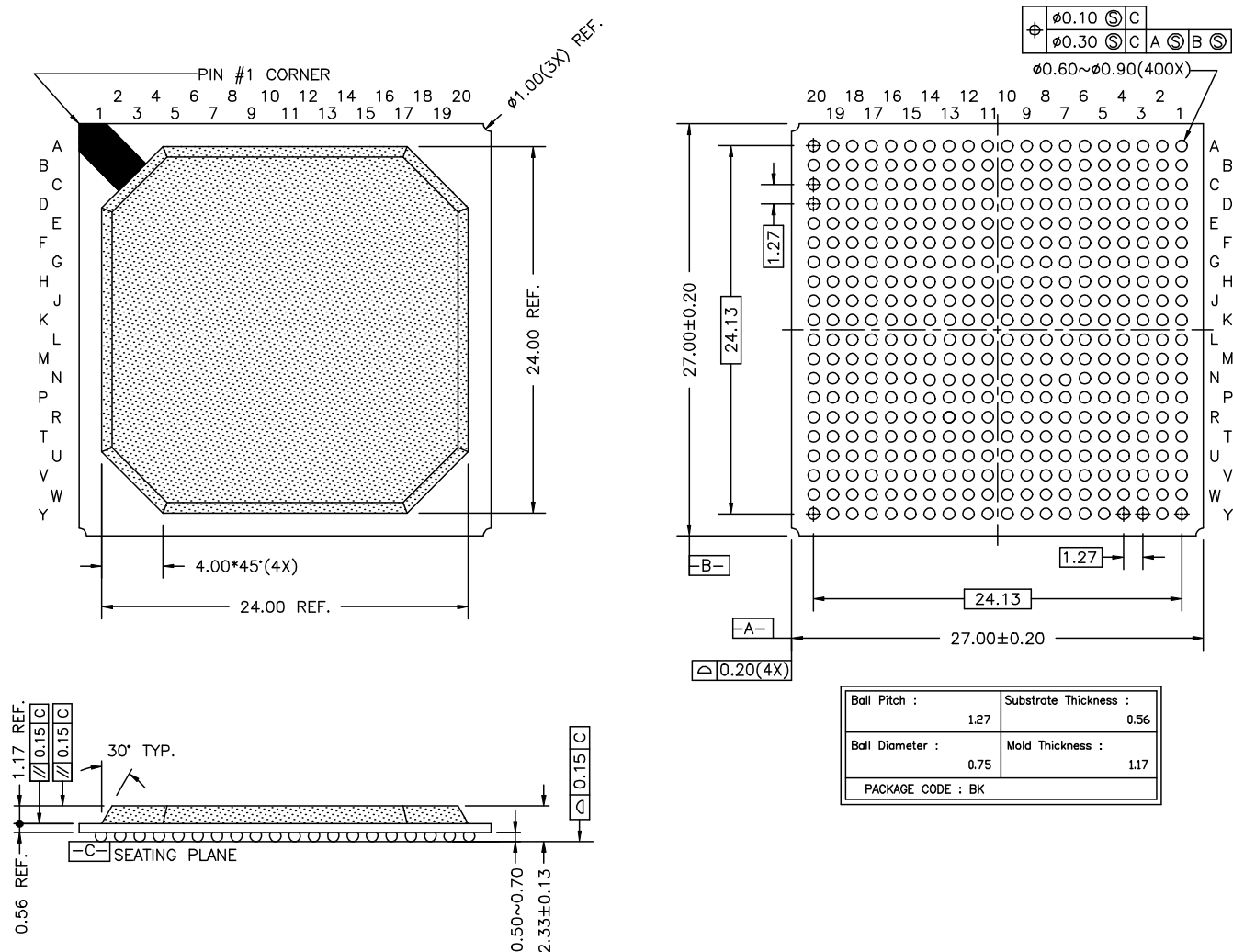
Figure 21. 400-Pin PBGA
