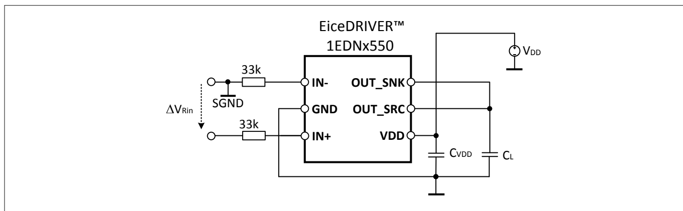
Figure 5 Test circuit
