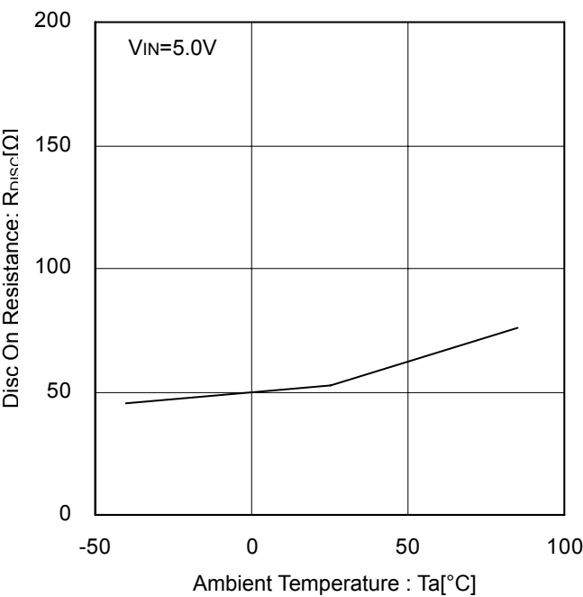
Figure 31. Discharge On Resistance vs Ambient Temperature
