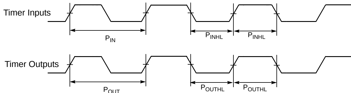
Figure 10-13 Timer Timing
