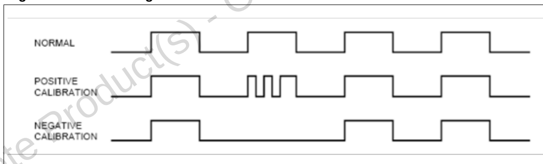
Figure 13. Calibrating waveform
