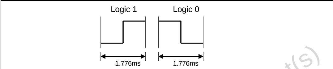
Figure 25. Bi-phase coding
