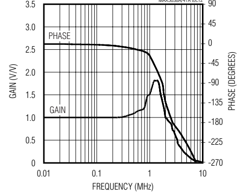
DIFFERENTIAL AMPLIFIER BANDWIDTH
