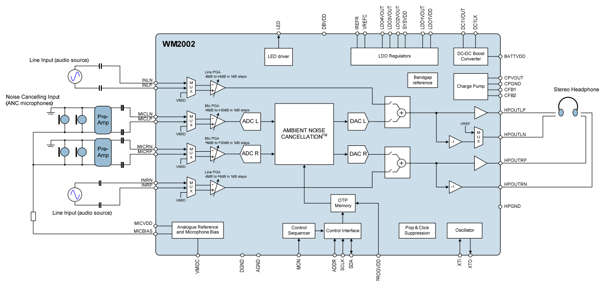
Figure 1 Typical Application
