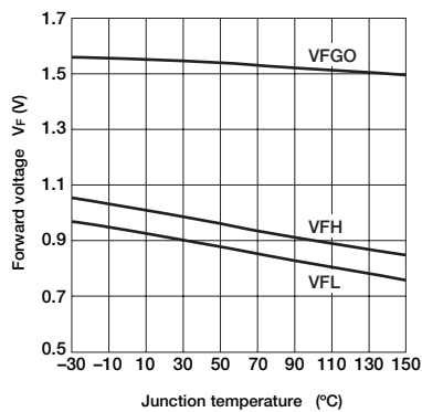
■ Diode V_f Characteristics ( I_f=0.5\text{A} )
