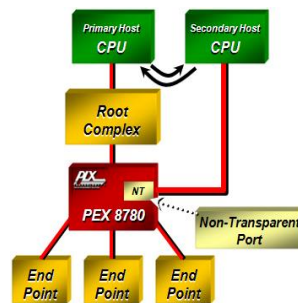
Figure 3: Non-Transparent Port
