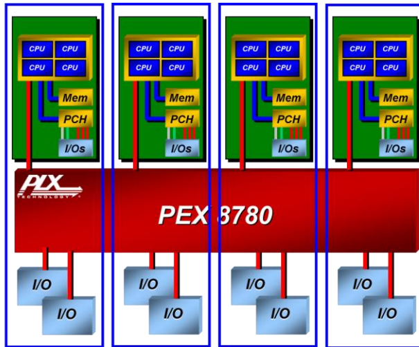
Figure 7. Multi-Host System
