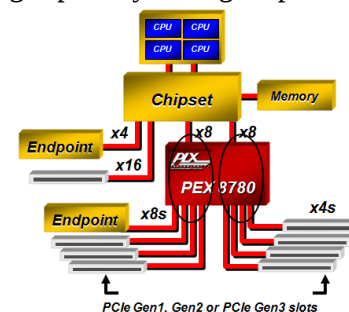
Figure 6. Host Centric Dual Upstream
