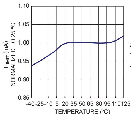
Peak Current Limit vs. Temperature
