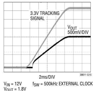
Ratiometric Tracking (Single Phase Using FDMF6707B DrMOS)
