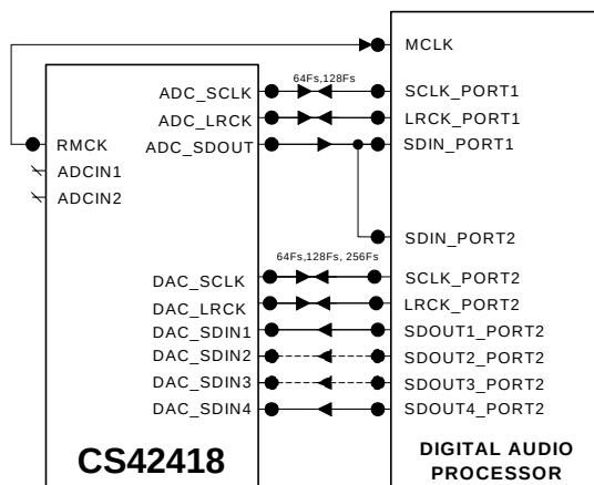
Figure 20. OLM Configuration #4
