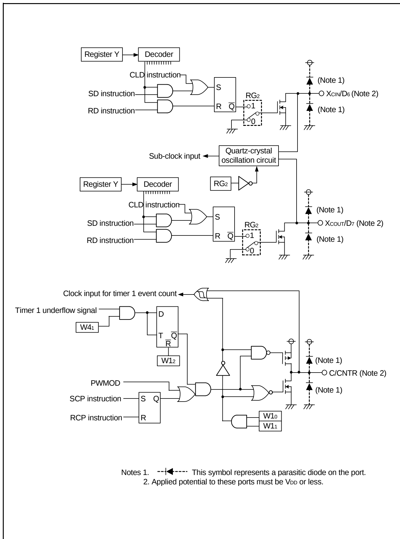
Fig 4. Port block diagram (2)
