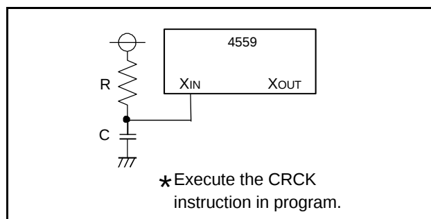
Fig 63. External RC oscillation circuit
