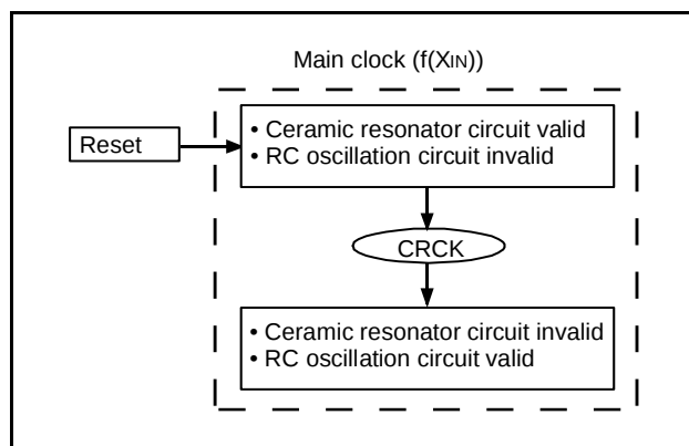
Fig 60. Switch to ceramic resonance/RC oscillation
