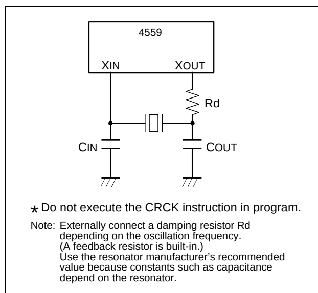
Fig 62. Ceramic resonator external circuit
