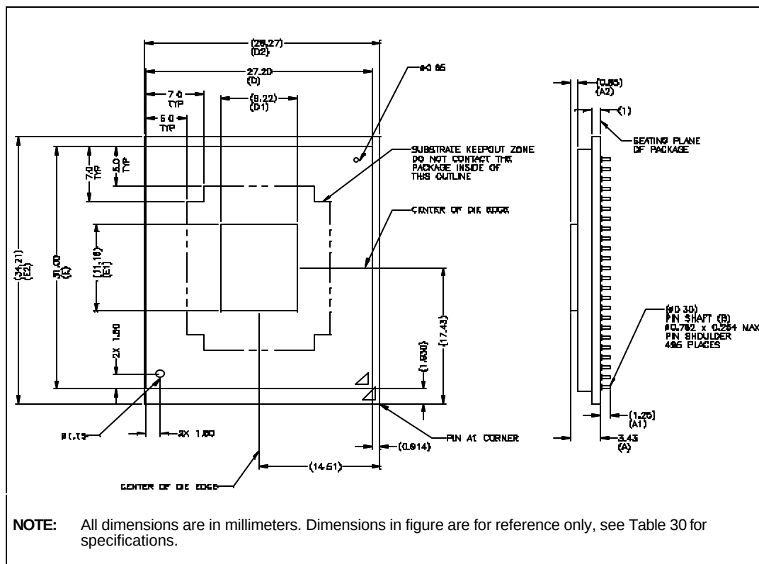
Figure 23. Socketable Micro-PGA2 Package - Top and Side View
