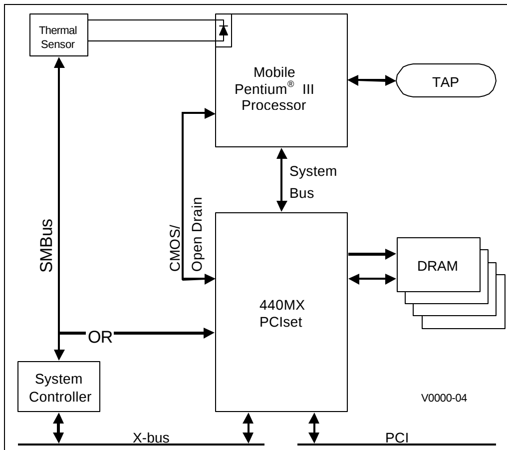
Figure 2. Signal Groups of a Mobile Pentium III Processor/440MX Chipset - Based System
