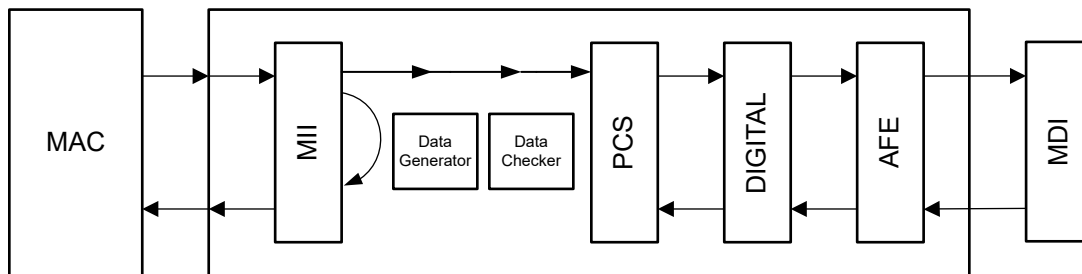
Figure 8-2. xMII Loopback Without Data Generator
