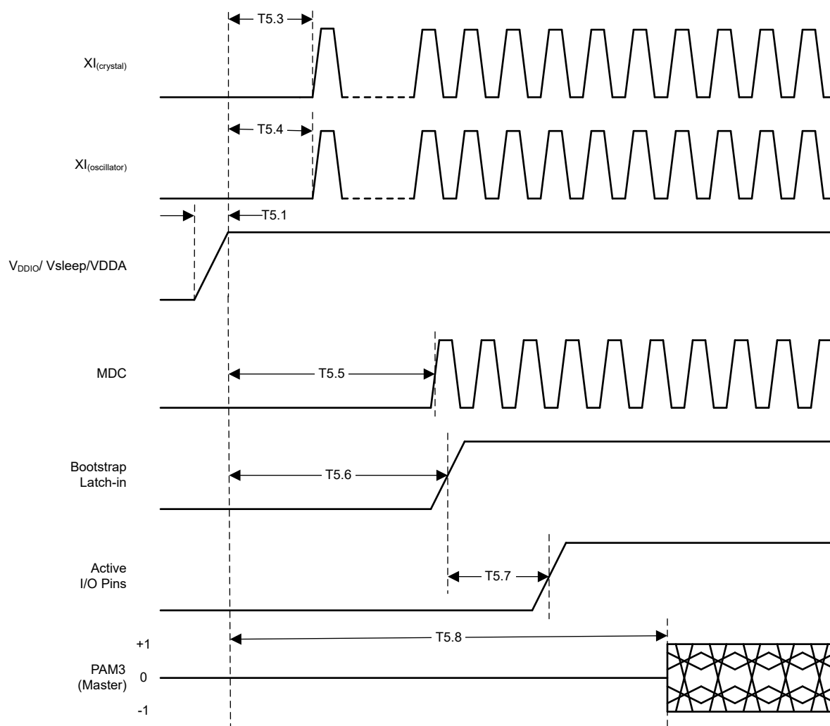
Figure 7-8. Power-Up Timing
