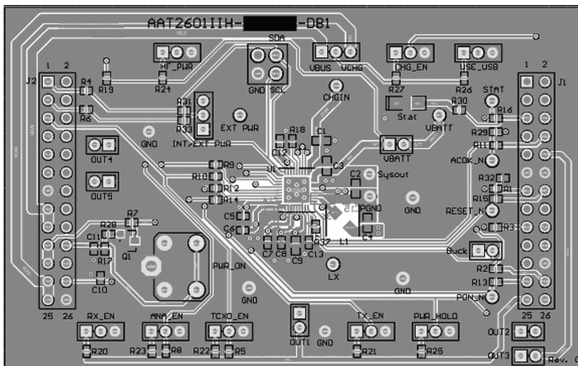
Figure 11: AAT2601B Evaluation Kit Top Layer.
