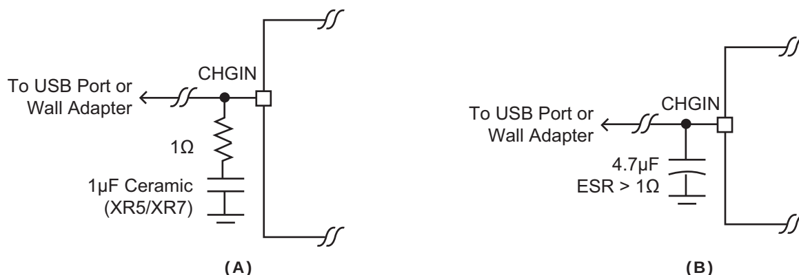
Figure 6: Hot Plug Requirements.
