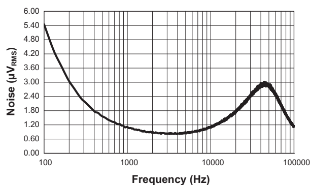
LDO Output Voltage Noise ( I_{OUT3} = 10mA , Power BW = 100~100KHz)
