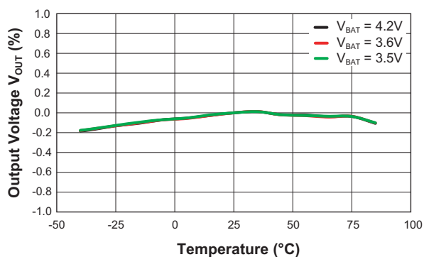
LDO1 Output Voltage vs. Temperature ( I_{OUT} = 10mA )
