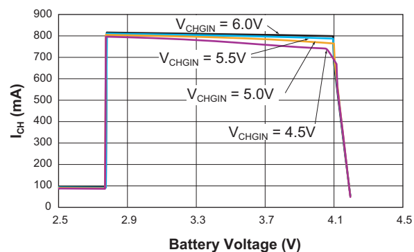
Charging Current vs. Battery Voltage ( R_{ISET} = 1.24k\Omega )
