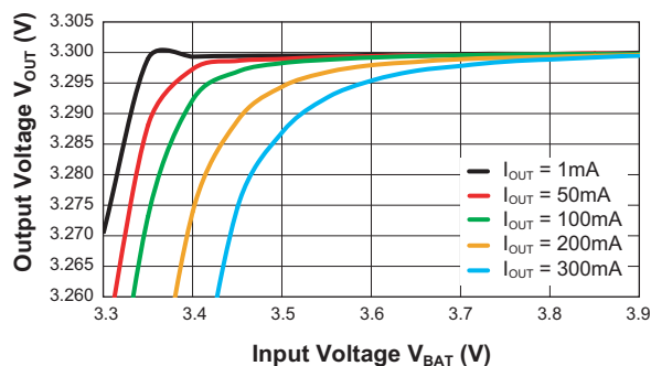
LDO1 Dropout Characteristics vs. Battery Input Voltage ( V_{OUT} = 3.3V )
