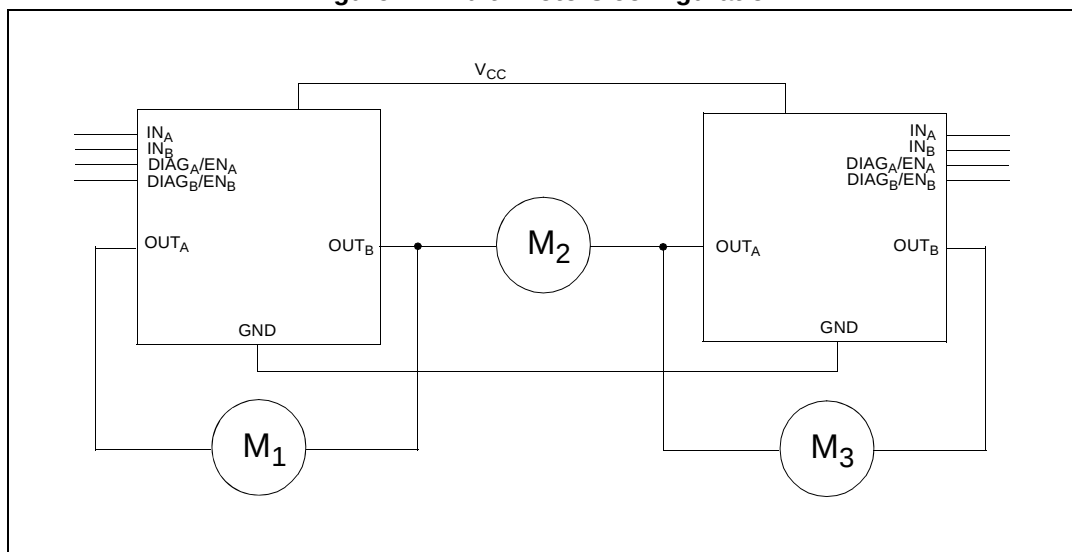
Figure 12. Multi-motors configuration
