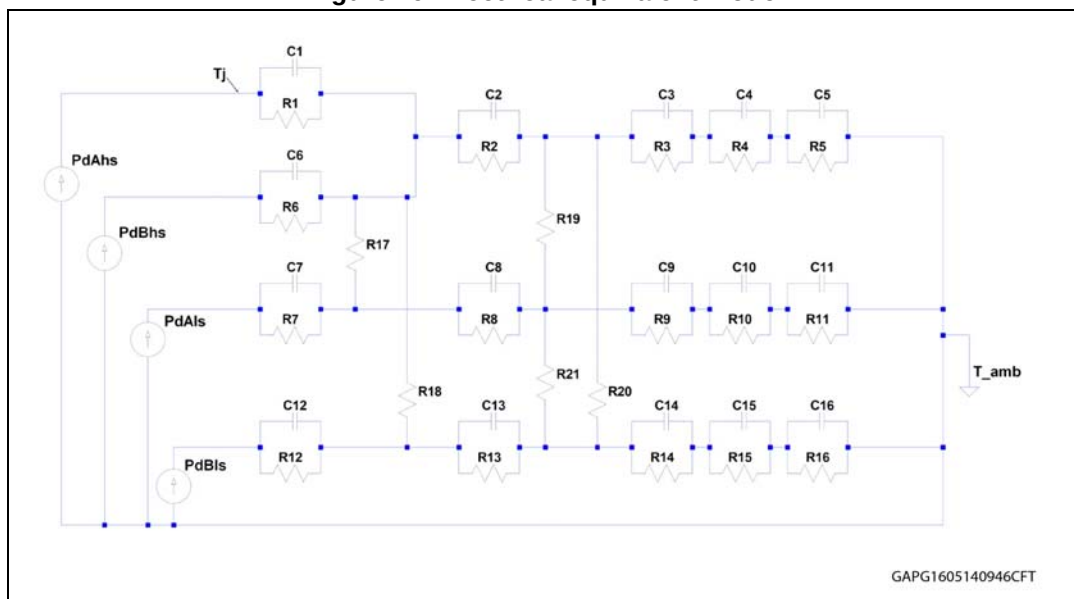
Figure 19. Electrical equivalent model
