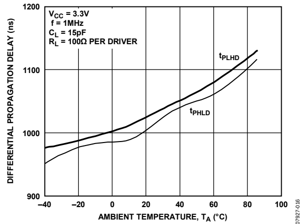
Figure 16. Differential Propagation Delay vs. Ambient Temperature
