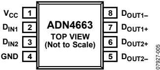
Figure 5. Pin Configuration
