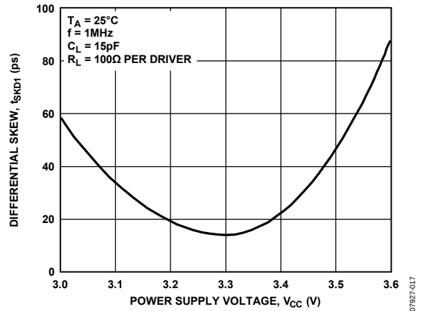
Figure 17. Differential Skew vs. Power Supply Voltage
