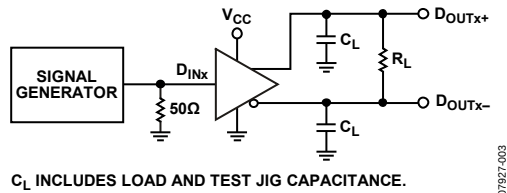
Figure 3. Test Circuit for Driver Propagation Delay, Transition Time, and Maximum Operating Frequency
