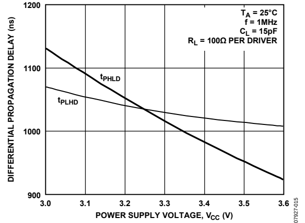
Figure 15. Differential Propagation Delay vs. Power Supply Voltage
